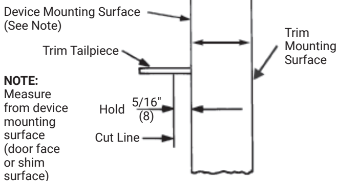
Figure 2: Tailpiece Sizing
