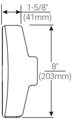
Cover Detail
