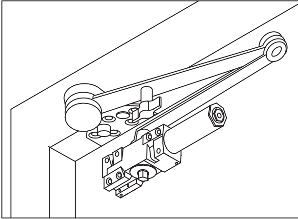
Standard Installation
