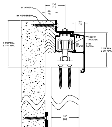
SHS80 Series Hardware Kit
