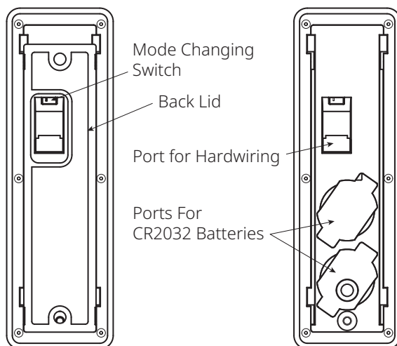
Figure 20: Wave Sensor
