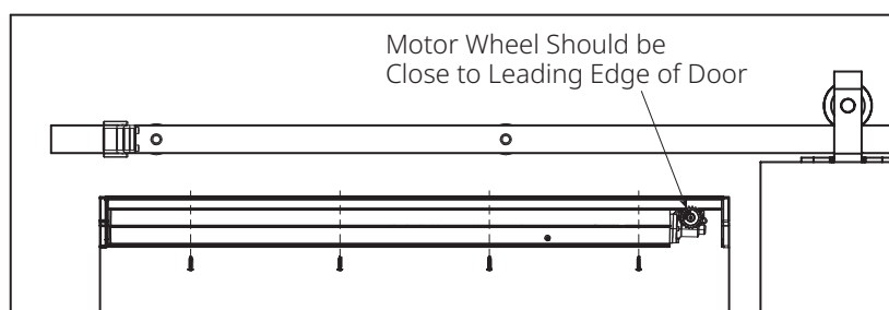
Figure 15: Mount the Unit Using the Provided Fasteners or Other Appropriate Fasteners
