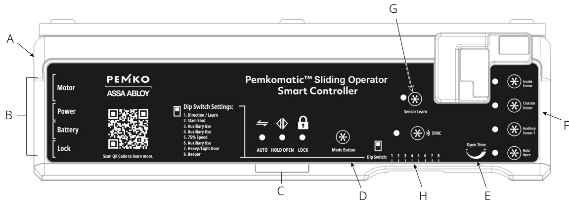
Figure 19: Control Panel
