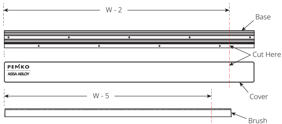
Figure 7: Cut Base, Cover, and Brushes
