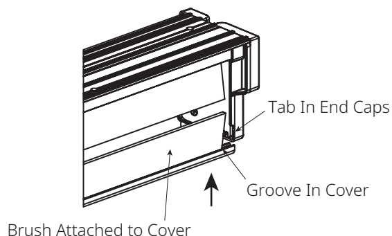
Figure 27: Align the Groove in Cover to the Tab on the End Caps
