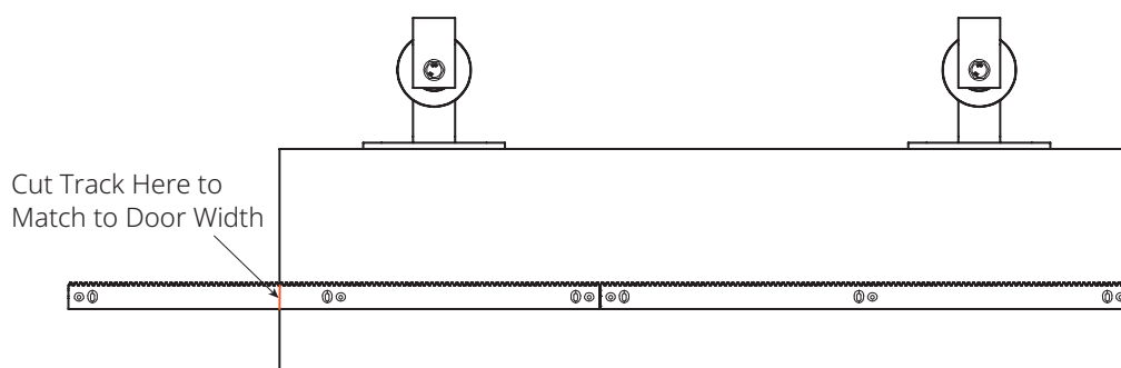
Figure 17: Length of Track = Width of the Door
