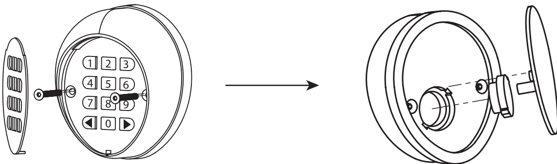
Figure 22: Install 2 CR2032 Batteries in the Keypad
