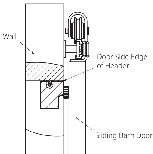
Figure 12: Sidewall Mount Sliding Door
