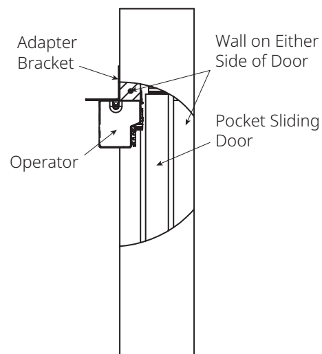
Figure 13: Pocket Sliding Door with Adapter Bracket
