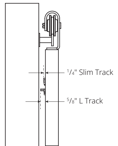
Figure 14: Track Dimensions
