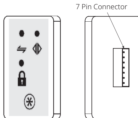
Figure 25: Connect other End of Cable to Mode Pad
