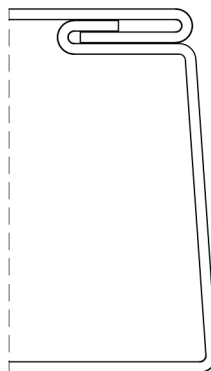
Continuous Interlocking Vertical Edge Seam
