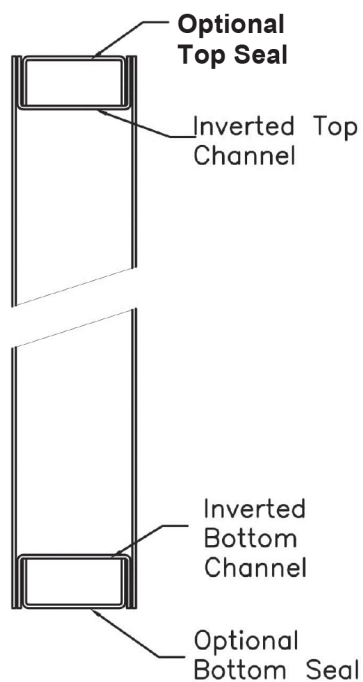
Top and Bottom Channels
